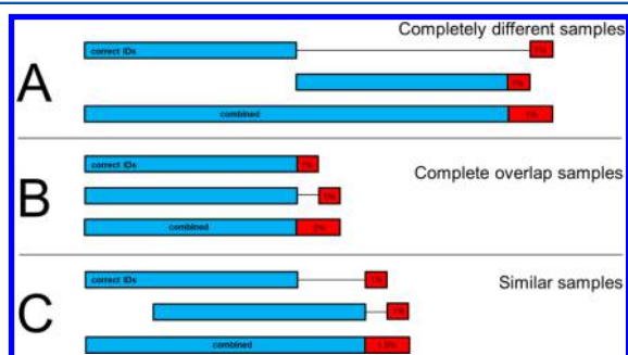
Figure 1. Three scenarios for how false discovery rates combine. True-positives are shown in blue and false-positives in red. The red false-positive boxes are depicted \sim 10 times larger than they should be for enhanced readability. (A) If none of the true-positives and 1% false-positives overlap, then the final FDR does not expand. (B) If all of the true-positives overlap but none of the false-positives overlap (because they are false and random), then the final FDR is double the original rates. (C) In a real-world scenario where the intersection of true-positives overlaps by 50% and the false-positives do not overlap, the combined FDR is 1.5%. This effect compounds as more data sets are merged.
